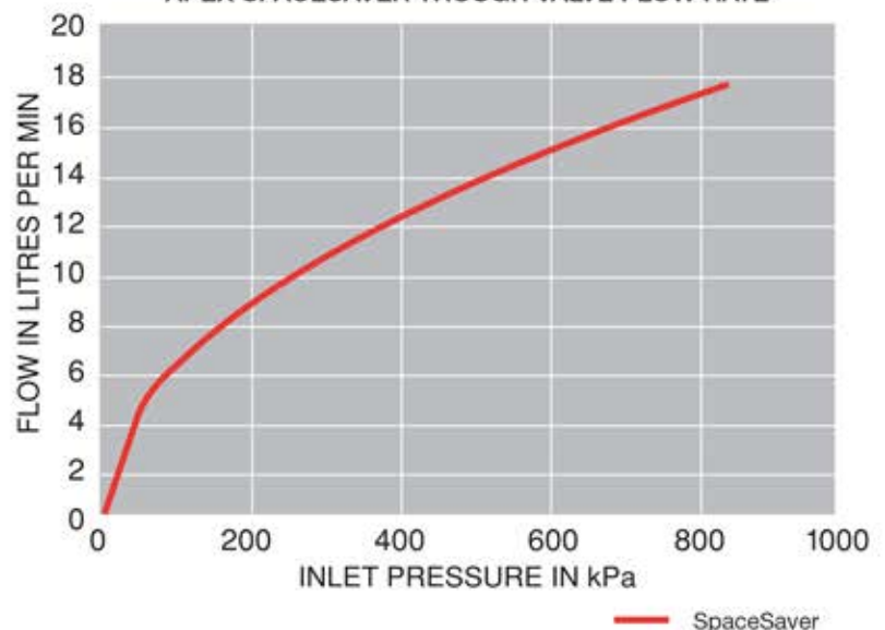
APEX SPACESAVER TROUGH VALVE FLOW RATE
