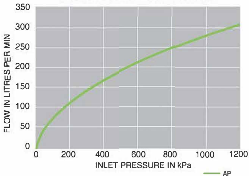
APEX ACETYL FULL FLOW VALVE FLOW RATE
